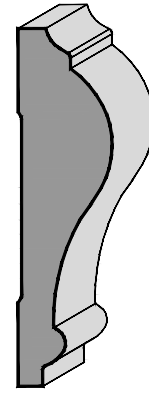
J832 1" x 3 3/4" (24.9 x 94.7mm)
