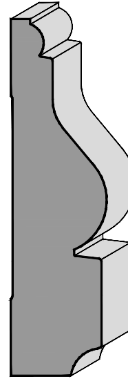
J1439 1\frac{7}{16}'' \times 5\frac{3}{8}'' (36.9 x 136.5mm)
