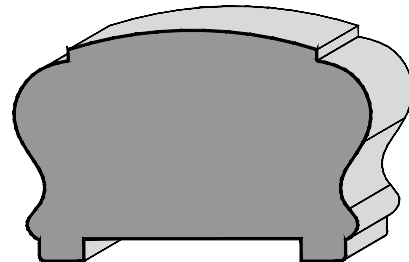
J953 3⅞" x 2⅜" (94.5 x 61.1mm)
